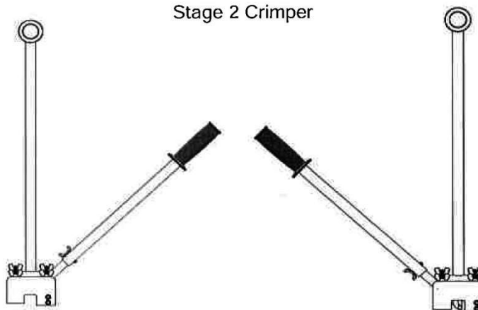
2-Stage Crimper
