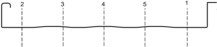
FASTENER SEQUENCE
