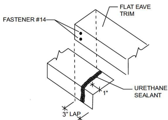
BOX PANEL CAP TRIM ENDLAP DETAIL
