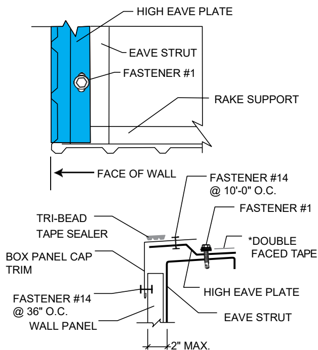
WALL PANEL INSTALLED BEFORE ROOF
