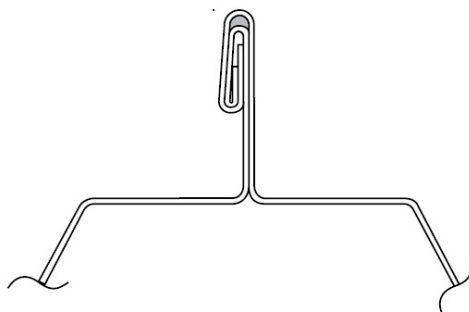
Cross Section of Finished Seam (Actual Size)
