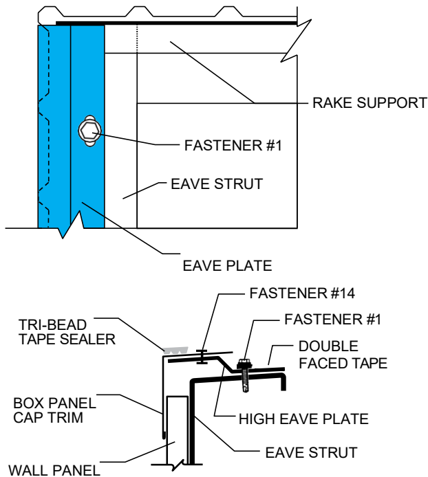
WALL PANEL INSTALLED BEFORE ROOF
