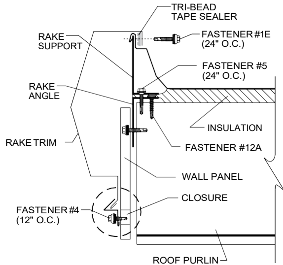
BEGINNING RAKE TRIM
