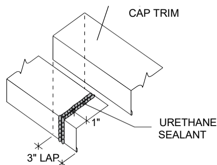
BOX PANEL CAP TRIM ENDLAP DETAIL
