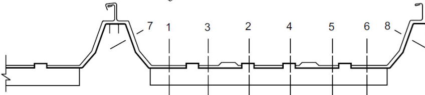
FASTENER SEQUENCE SUBSEQUENT RUNS - ENDLAP
