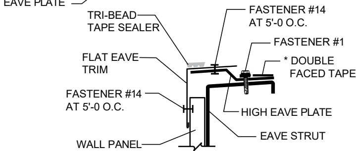
WALL PANEL INSTALLED BEFORE ROOF (FIXED EAVE)
