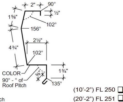
Sculptured Eave Trim
