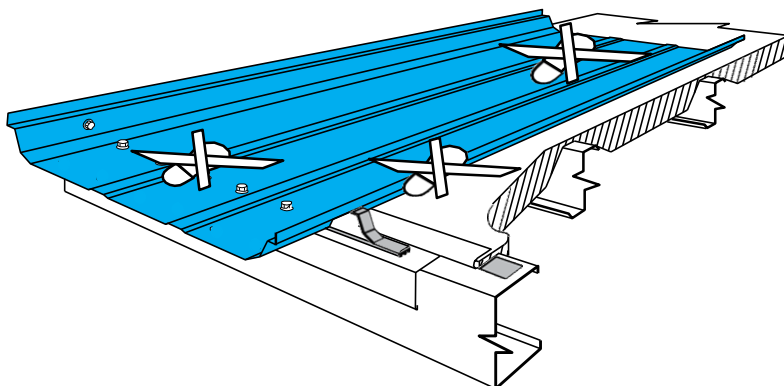
FASTENER SEQUENCE FIRST RUN - EAVE
