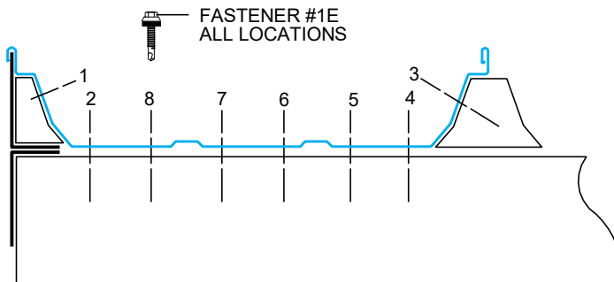
FASTENER SEQUENCE FIRST RUN - EAVE
