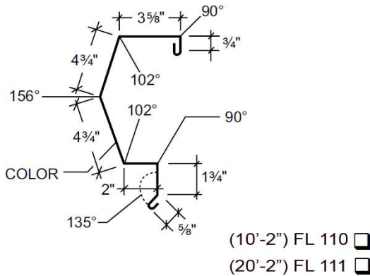
Sculptured Eave Trim
