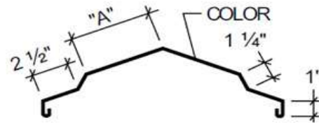
Ridge Flashing - For Ridge Vent
