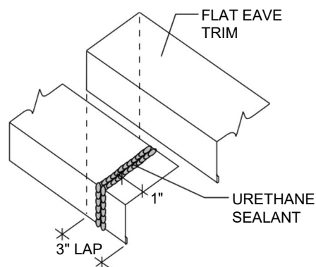
FLAT EAVE TRIM ENDLAP DETAIL
