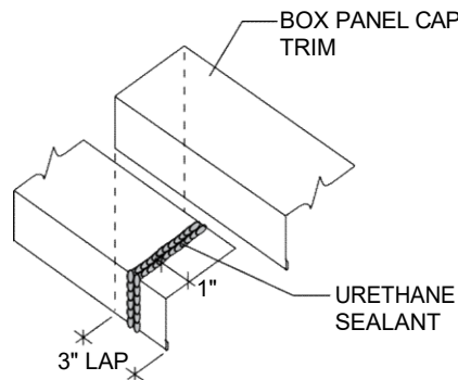
BOX PANEL CAP TRIM ENDLAP DETAIL
