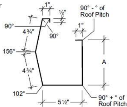
Sculptured Gutter
